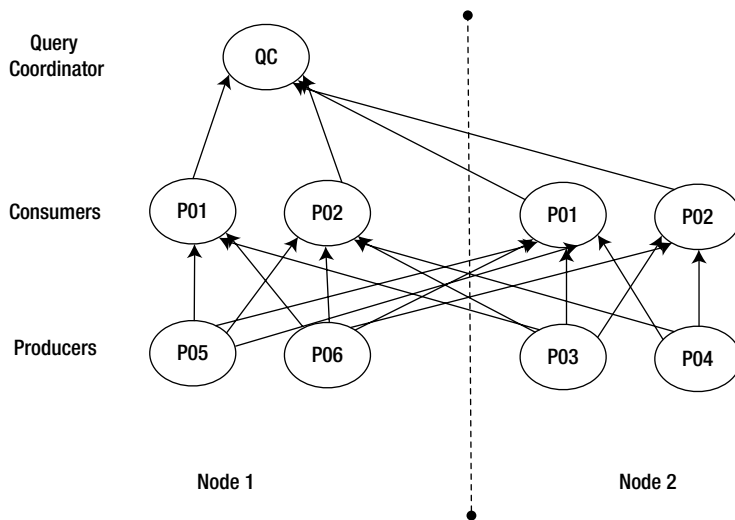
Figure 12-3. PX execution in RAC
