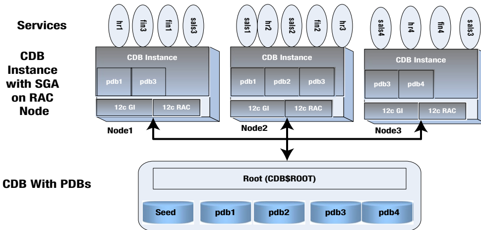
Figure 4-10. Oracle RAC-based CDB
