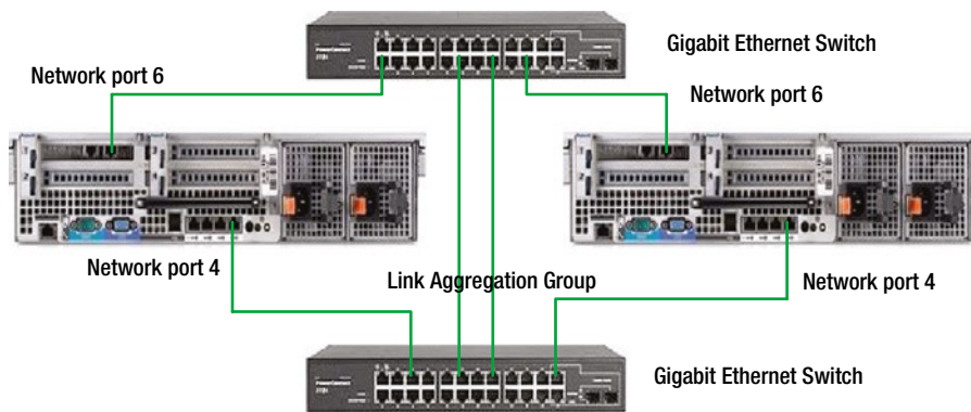
Figure 9-9. A fully redundant private network configuration
