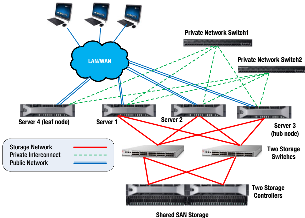
Figure 1-2. Oracle RAC hardware architecture
