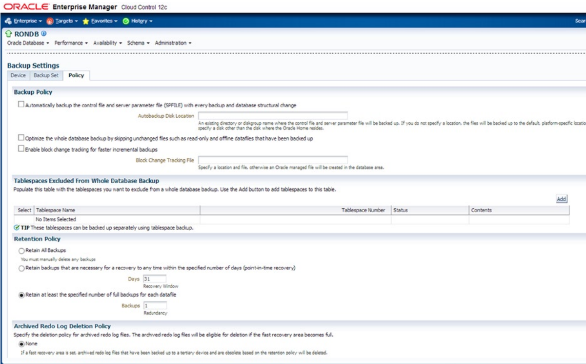
Figure 8-9. OEM Cloud Control 12c Backup_setting_policy screen
