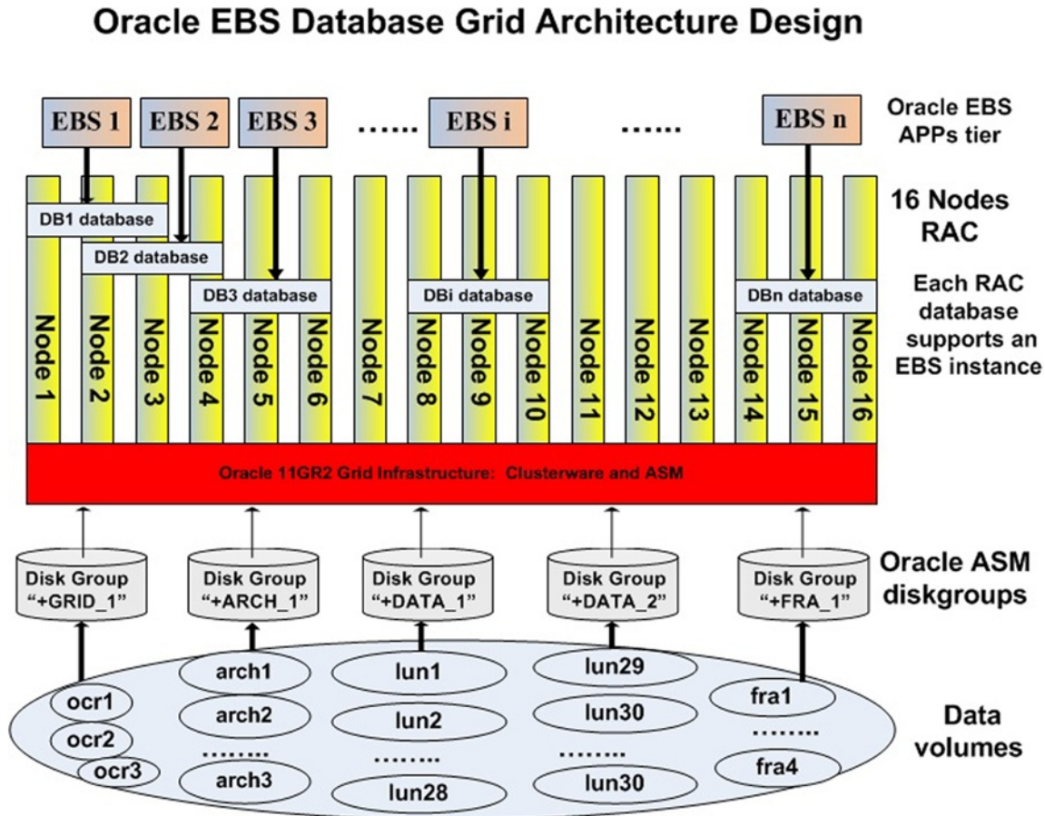
Figure 1-5. The shared infrastructure for database consolidation
