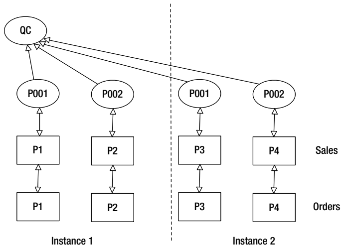
Figure 12-4. Partition-wise join
